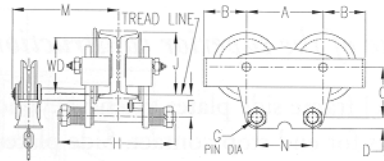
Hand-Geared Trolley 1/2, 1, 2 & 3 Ton
